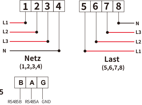
Abb. 7.22 EASTRON-Messer
