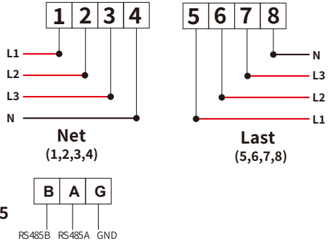
Abb. 7.1 EASTRON-Messer
